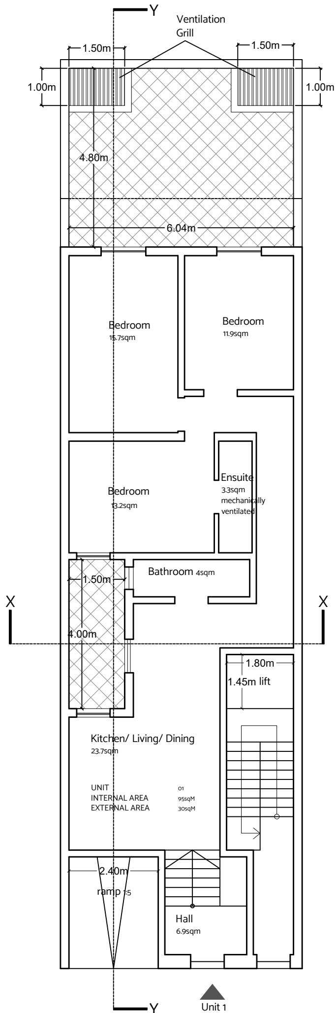
Proposed Elevated Ground Floor Scale 1:100
